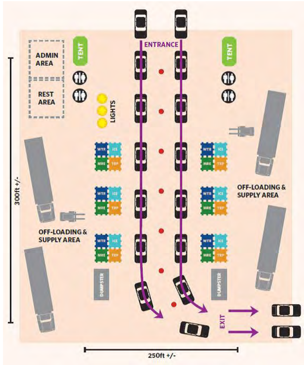
Figure H.4-3. Type II Vehicular POD layout.
